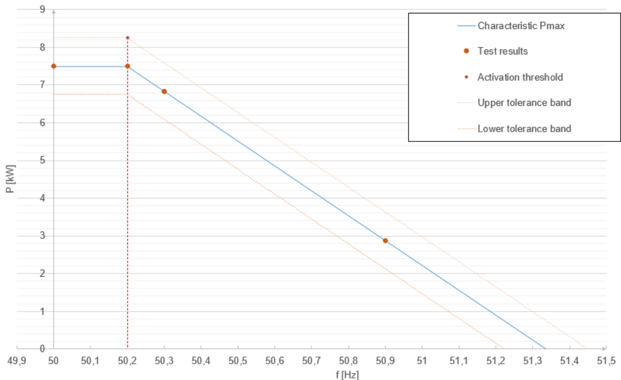
Figure 5-4 LFSM-O test result, showing test results (orange dots) compared to required droop characteristic (blue line), droop:5%, activation threshold: 50,2 Hz, Based on data from /1/
